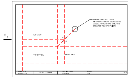
MAKE CONSTRUCTION LINES - 7
