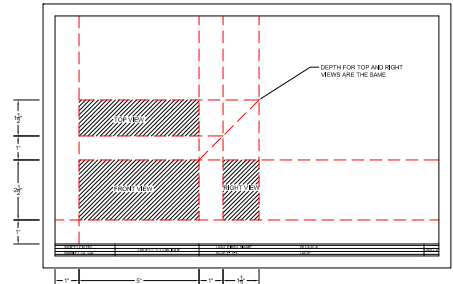
DRAW VIEWS IN SHADED AREAS
