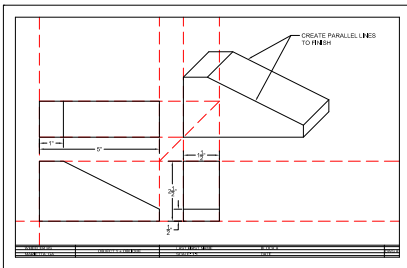
MAKE PICTORIAL - OBLIQUE - 4
